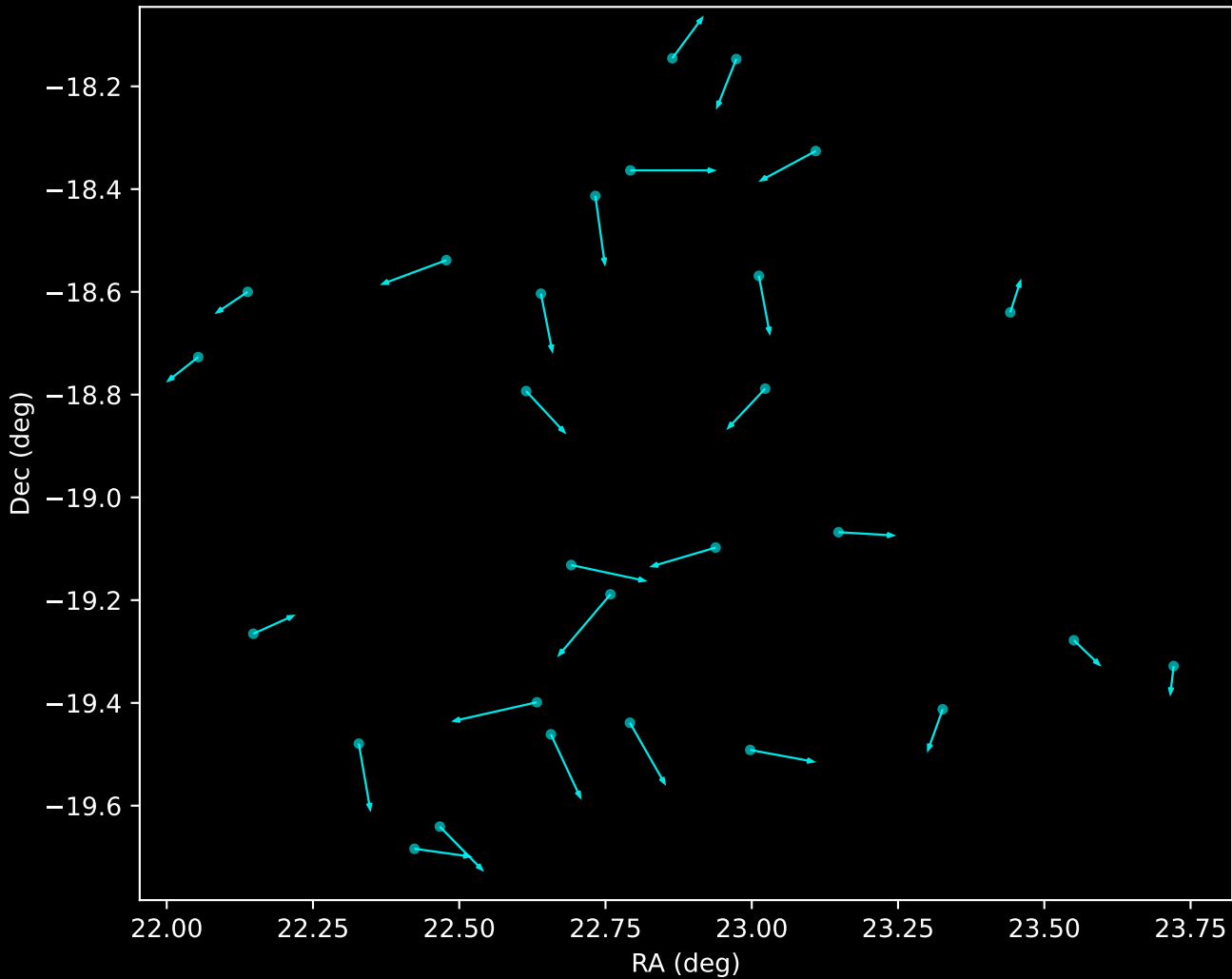
APOGEE DR17 Noise Stream Proper Motion Vectors (n=28)
