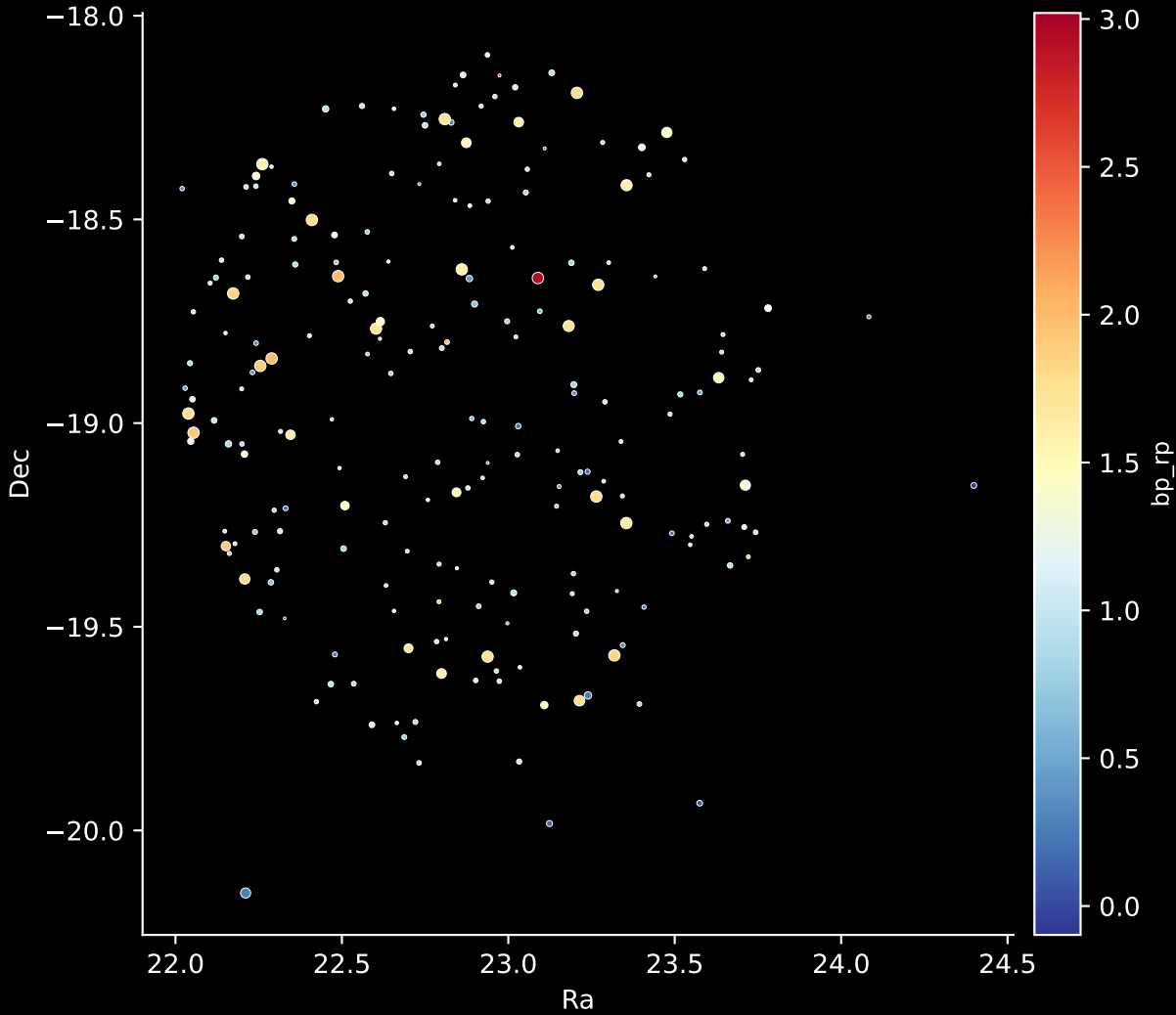
APOGEE DR17 Field: [K2_C7_016-09_btx] Stars: 208
