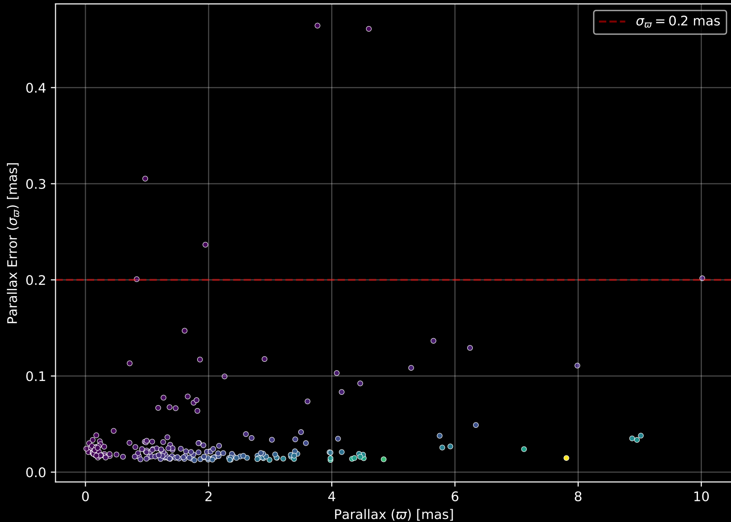
APOGEE DR17 Field: [K2_C7_016-09_btx] Parallax Quality (n= 208)
