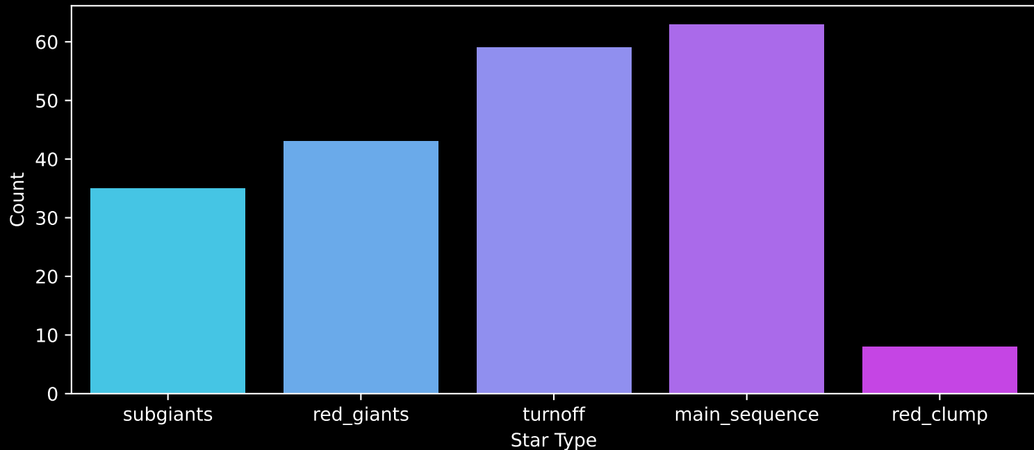
APOGEE DR17 Field: [K2_C7_016-09_btx] Count plot of Star Type
