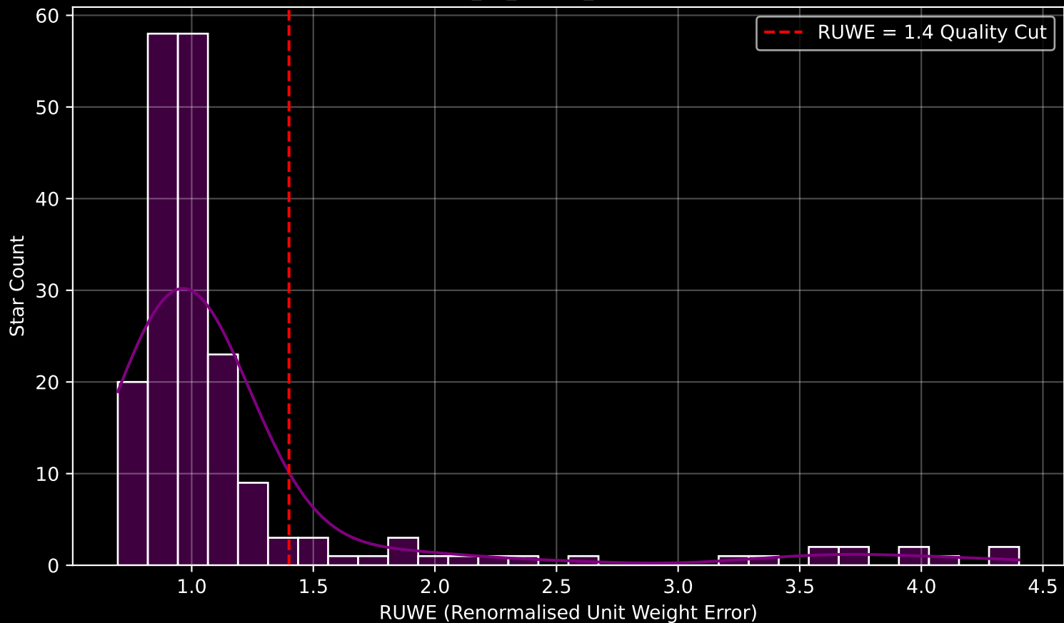
GAPOGEE DR17 Field [K2_C7_016-09_btx] RUWE Distribution (n= 195)
