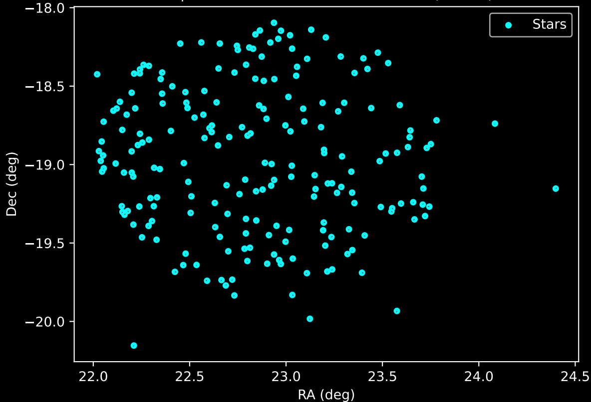
APOGEE DR17 Field: [K2_C7_016-09_btx] Proper Motion Vectors for Gaia Star Field (n= 208)
