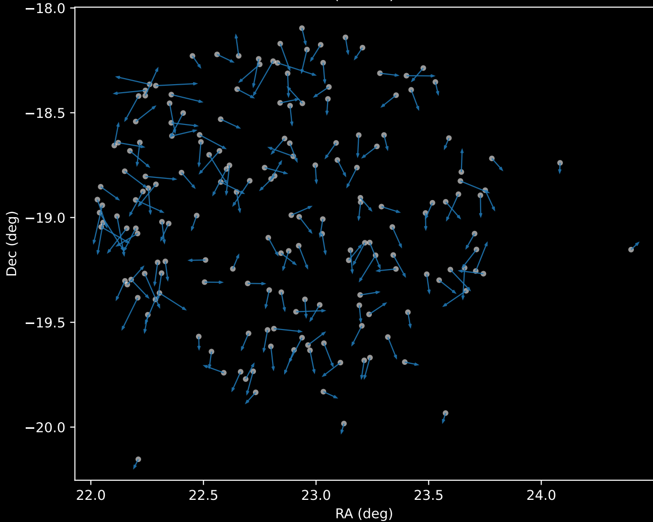
APOGEE DR17 Cluster 0 Proper Motion Vectors (n=175)
