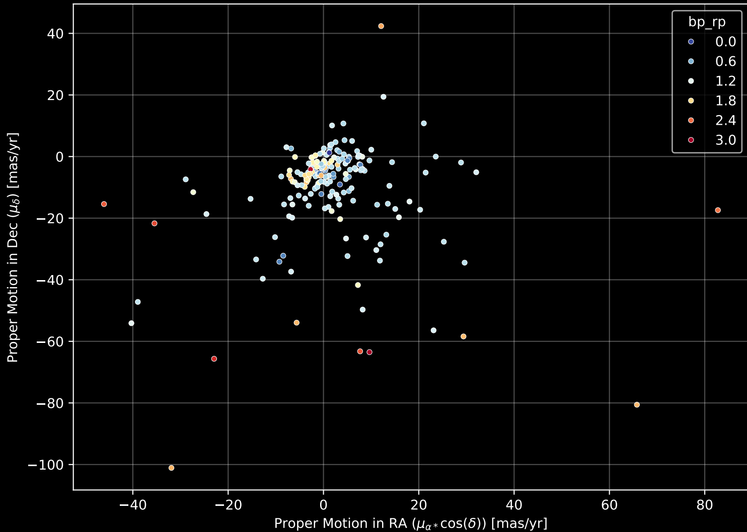
APOGEE DR17 Field: [K2_C7_016-09_btx] Proper Motion Diagram (n= 208)
