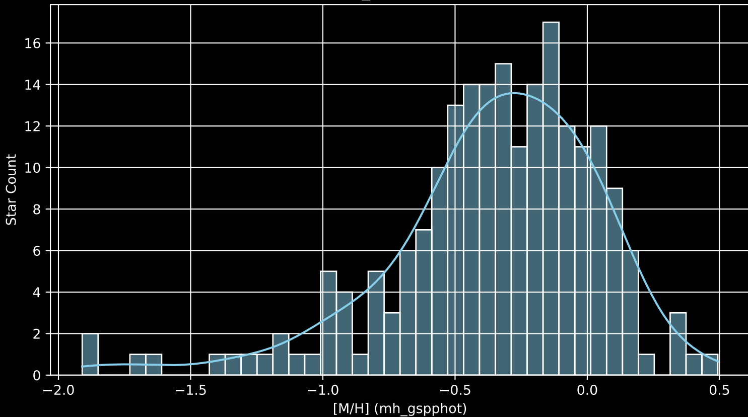
APOGEE DR17 Field: [K2_C7_016-09_btx [M/H] (mh_gspphot) (n= 207)
